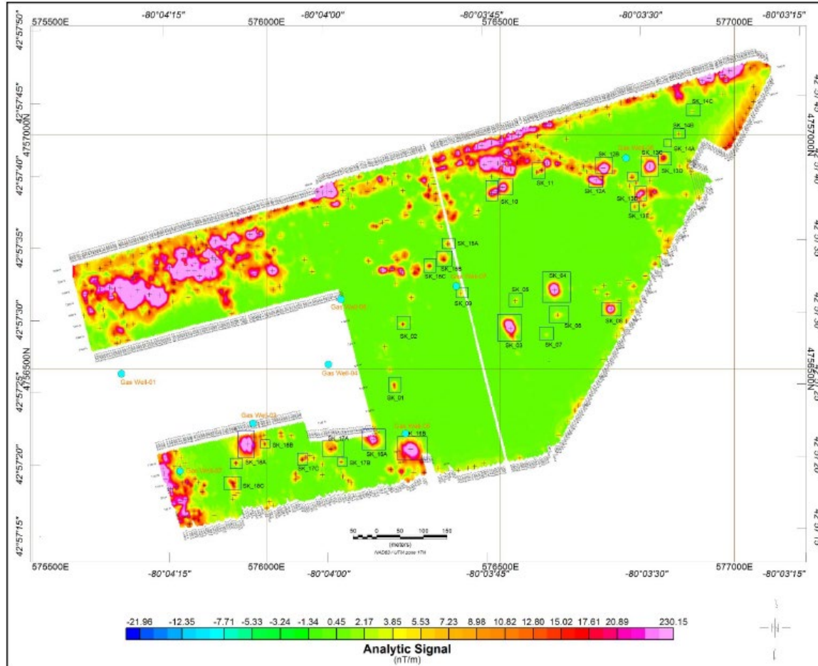
Using drone-MAG surveying.
